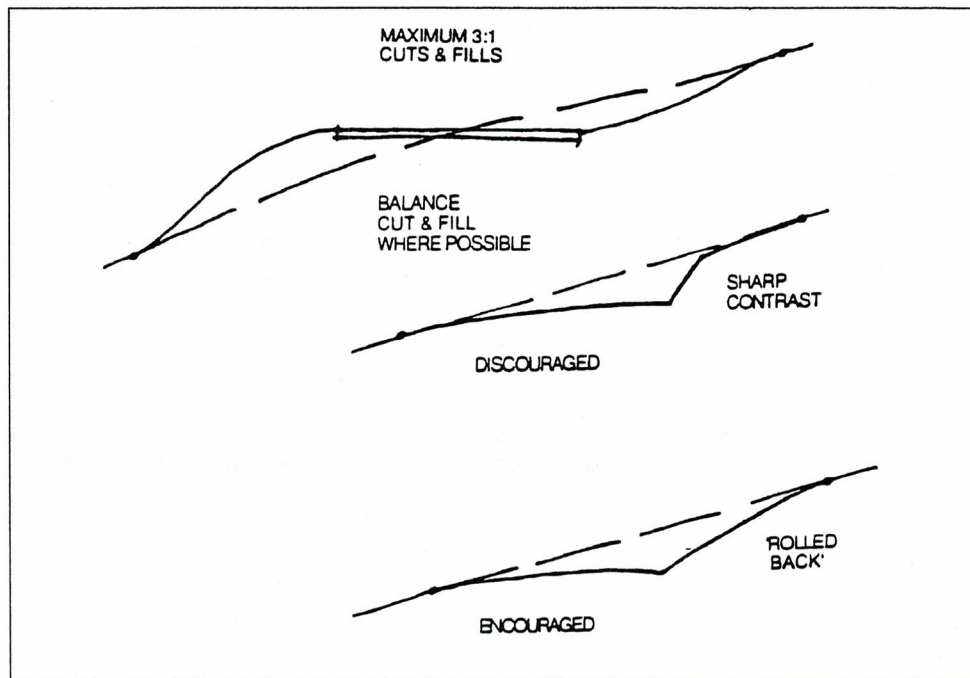
Fig. 1—Erosion Control
